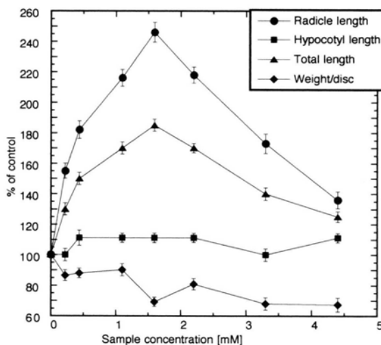
Fig. 1. The effects of various concentrations of 8-desacylvernolol ( 1 ) on the growth of lettuce seeds after 72 h of incubation in the dark at 24 °C (control lengths: radicle = 11 mm, hypocotyl = 9 mm, total length = 20 mm).
